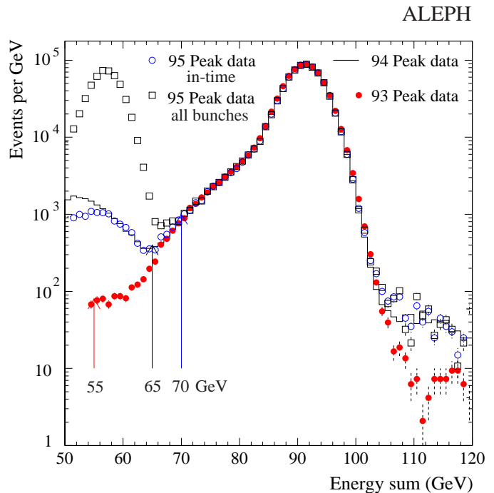
Fig. 3. SICAL energy sum distribution for clusters satisfying radial and azimuthal requirements. The different levels of beam-related background and the bunch train operation in 1995 necessitated the evolution of the cut on the energy sum as indicated by the arrows
