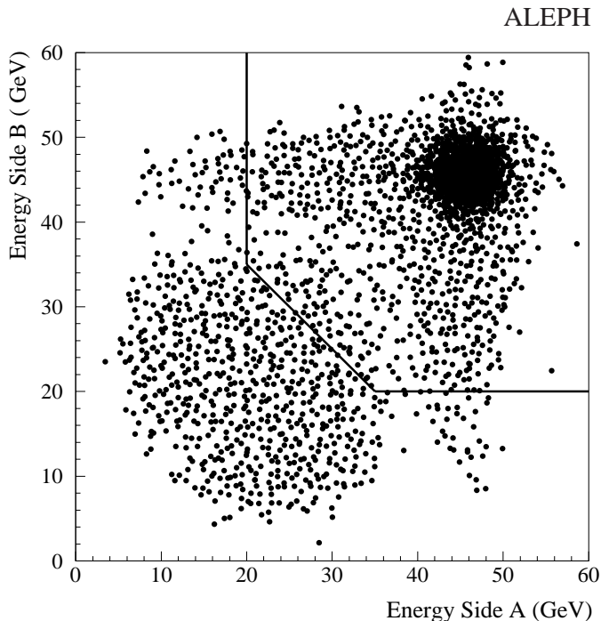
Fig. 2. SICAL highest reconstructed cluster energy on side A versus highest reconstructed cluster energy on side B for clusters satisfying radial and azimuthal requirements. The entries around 20 GeV originate from accidental coincidences of off-momentum beam particles. More than 99.9% of the Bhabha events satisfy the energy cut requirements
