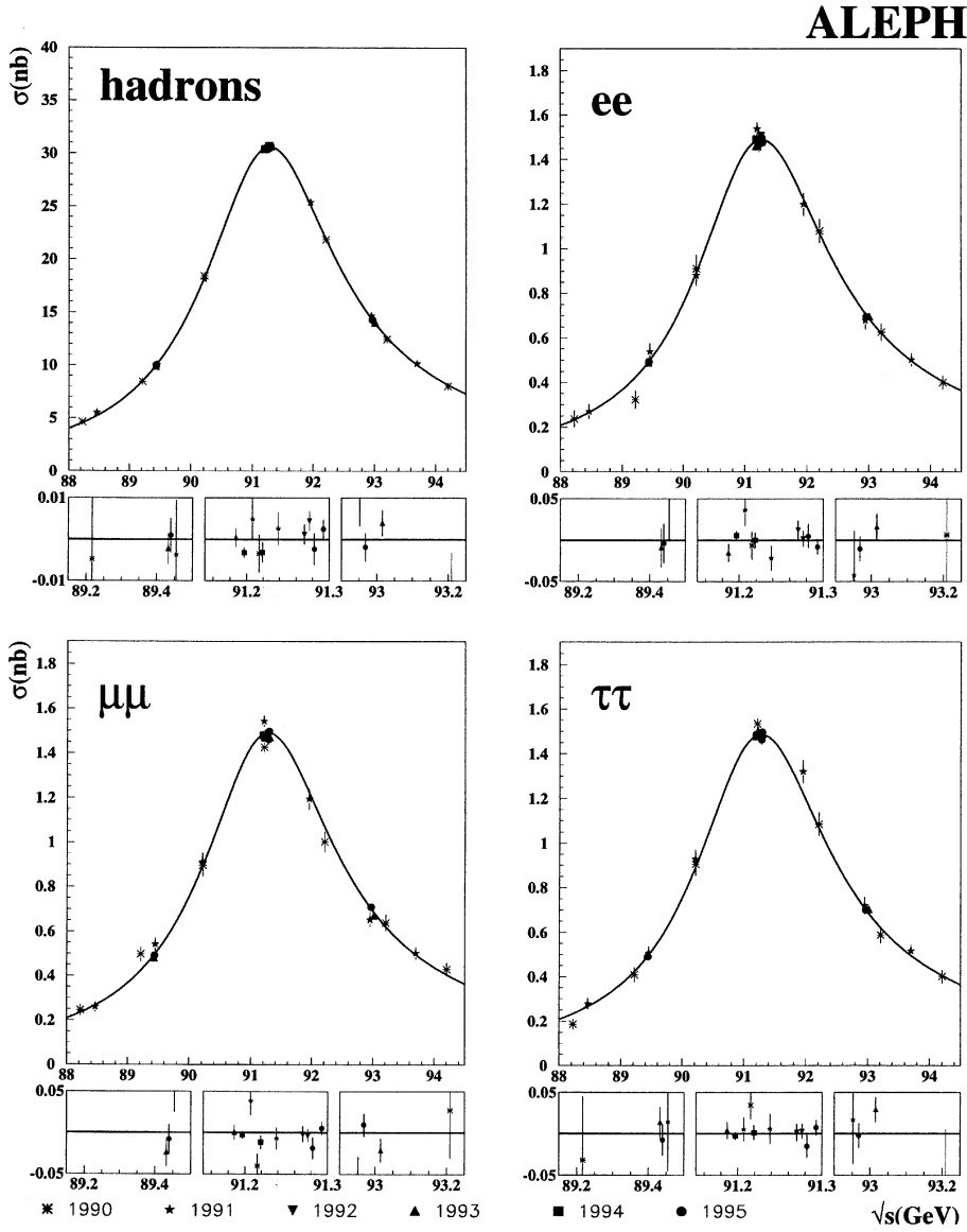
Fig. 21. Measurement of cross sections. The solid lines show the result of the Standard Model fit. The inserts show enlarged views of the peak, peak-2 and peak+2 regions for the relative difference between data and fit
