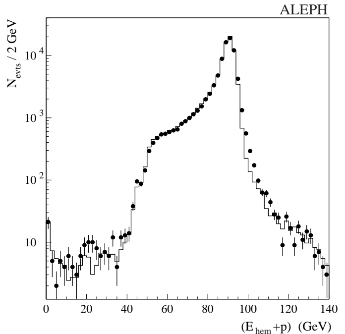
Fig. 17. Global selection: E_{\text{hem}} + p for Bhabha-like hemispheres in data (points) and Bhabha Monte Carlo (histogram)
