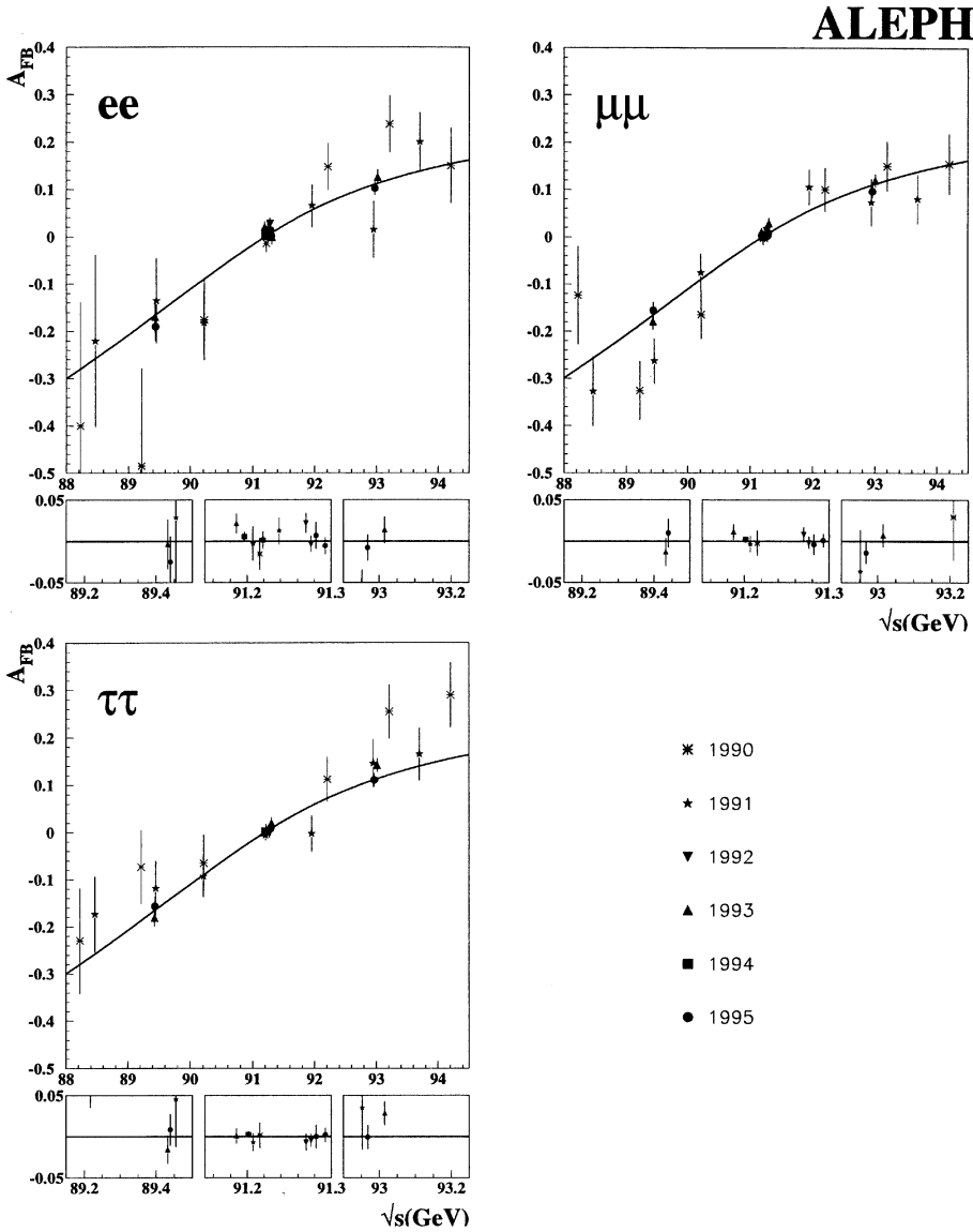
Fig. 22. Measurements of forward-backward asymmetries. The solid lines show the results of the Standard Model fit. The inserts show enlarged views of the peak, peak-2 and peak+2 regions for the difference between data and fit
