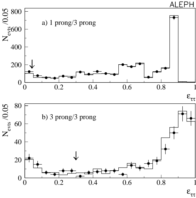
Fig. 15a,b. Global selection: distribution of the normalised estimator \mathcal{E}_{\tau^+\tau^-} a for artificial one-prong/three-prong events and b three-prong/three-prong events. The points represent the data, and the histogram the \tau^+\tau^- Monte Carlo. The arrows indicate the position of the cuts
