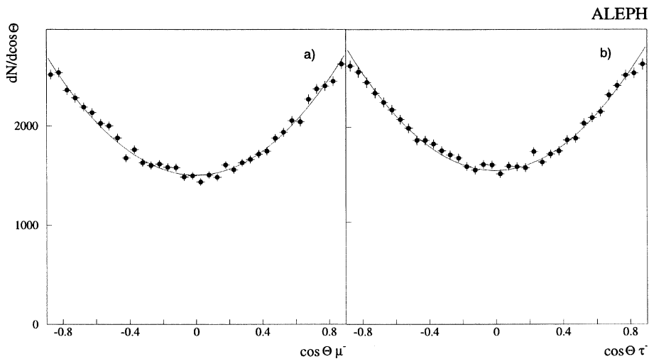
Fig. 20a,b. Angular distributions of the negative lepton at the peak energy in 1994, for muons a and taus b . The curves are the result of the maximum likelihood fits. The loss of efficiency at large |\cos\theta| comes from the angular acceptance cut
