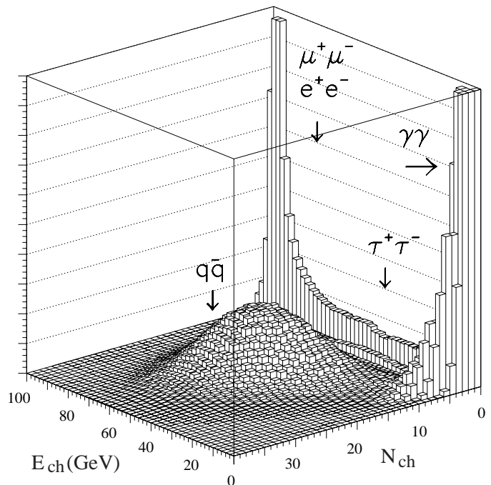
Fig. 4. Distribution of charged multiplicity N_{ch} versus charged-track energy E_{ch} for events passing the Z triggers
