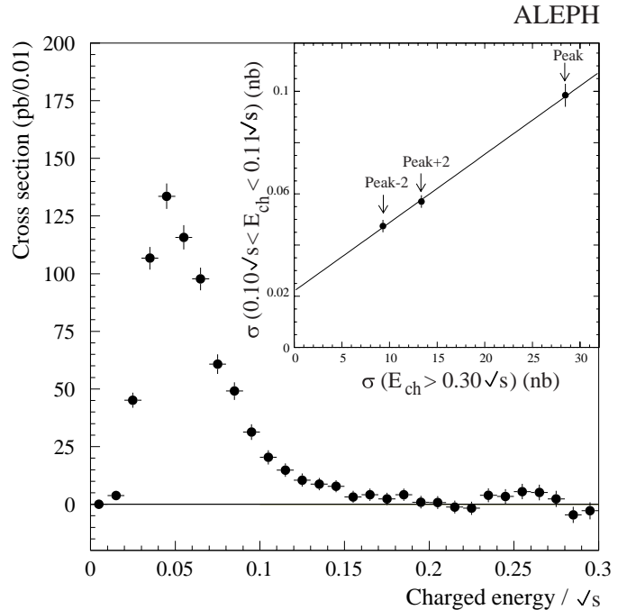
Fig. 6. Observed non-resonant hadronic cross section as a function of the normalised charged-track energy. Insert: total hadronic cross section in the charged-track energy interval (0.10,0.11)\sqrt{s} as a function of the cross section for events with charged-track energy greater than 0.3\sqrt{s} at three different centre-of-mass energies (peak-2, peak+2, peak). The offset of the straight line fit is the non-resonant contribution for the energy interval (0.10,0.11)\sqrt{s}
