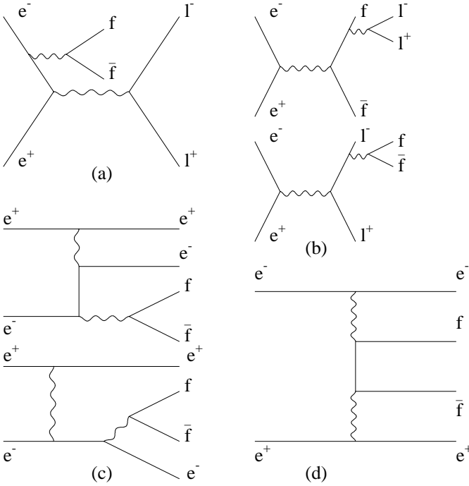
Fig. 8a–d. Diagrams contributing to llV processes
