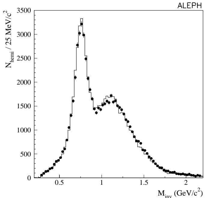
Fig. 13. Global selection: invariant mass of hadronic hemispheres classified as mh+n\pi^0 with m+n \geq 2 . The points represent the data, and the histogram the \tau^+\tau^- Monte Carlo
