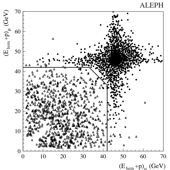
Fig. 16. Global selection: E_{\text{hem}} + p in hemisphere 1 versus hemisphere 2 for events identified as \mu/\mu . The triangles represent the \tau^+\tau^- Monte Carlo, the full circles the \mu^+\mu^- Monte Carlo. The lines indicate the cuts that define the \mu^+\mu^- sample
