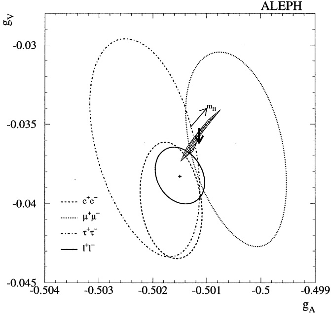
Fig. 24. Shown are the one- \sigma contours (39.3% CL). The shaded area indicates the Standard Model expectation for M_t = 174 \pm 5 \text{ GeV}/c^2 and 90 < M_H/\text{GeV}/c^2 < 1000 ; the vertical arrow shows the change if the electromagnetic coupling constant is varied within its error. This figure shows that the data favour a light Higgs boson
