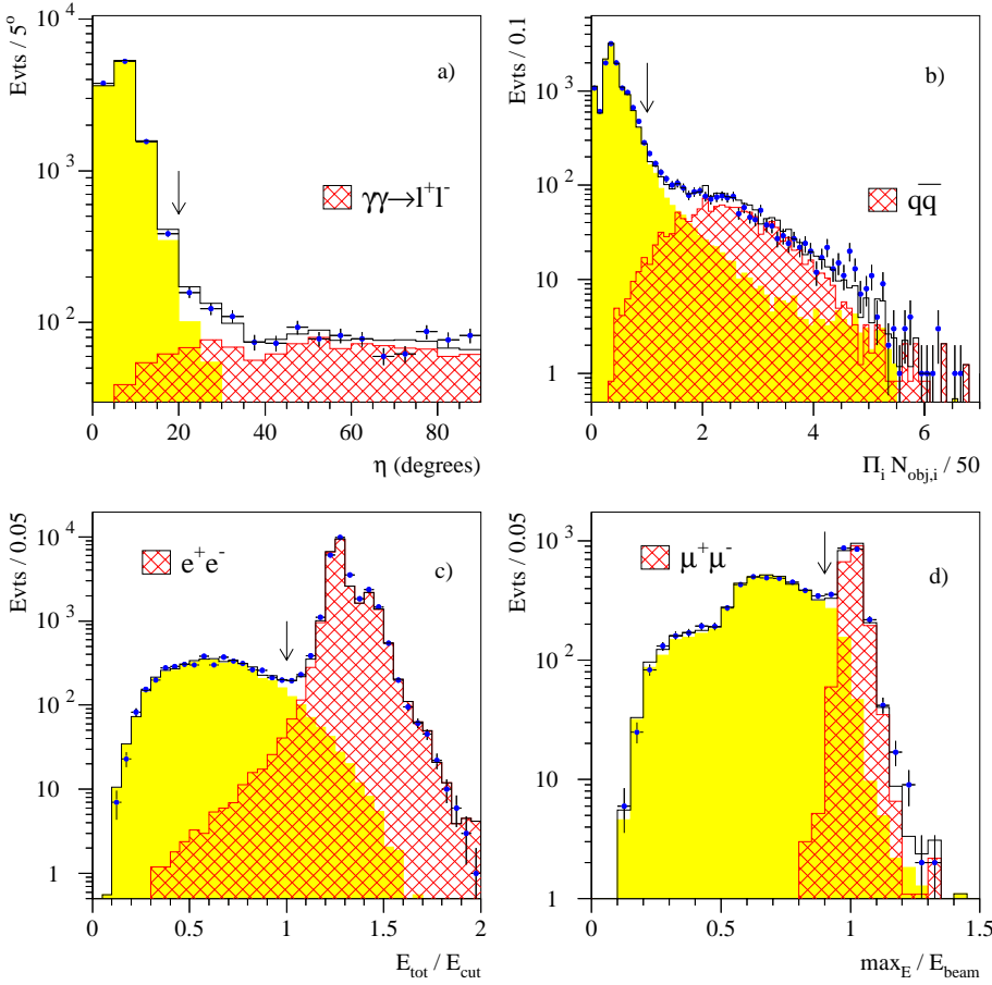
Fig. 10a–d. Exclusive \tau^+\tau^- selection: distribution of some of the variables used in the selection; see text for the description of the variables. The dots represent the 1994 data, the shaded areas the \tau^+\tau^- Monte Carlo and the crossed-hatched areas the dominant background rejected by the cut on the displayed variable. a Acollinearity for events selected by applying all the other selection cuts; b N_1^{\text{obj}}N_2^{\text{obj}} for q\bar{q} -like events, normalised to the value of the cut applied; c E_{\text{tot}} for Bhabha-like events, normalised to the value of the cut applied; d \max_E for dimuon-like events. The arrows indicate the position of the cuts
