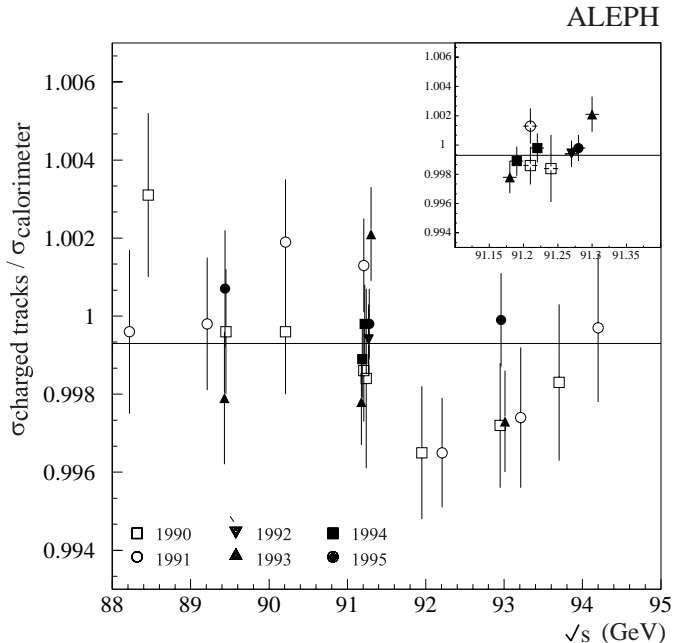
Fig. 7. Ratio of cross sections of the two hadronic selections as a function of centre-of-mass energy. The insert is an enlargement of the measurements around the Z peak
