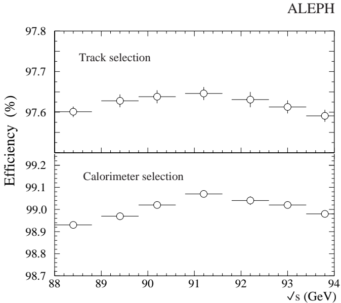
Fig. 5. Efficiency as a function of centre-of-mass energy for both selections
