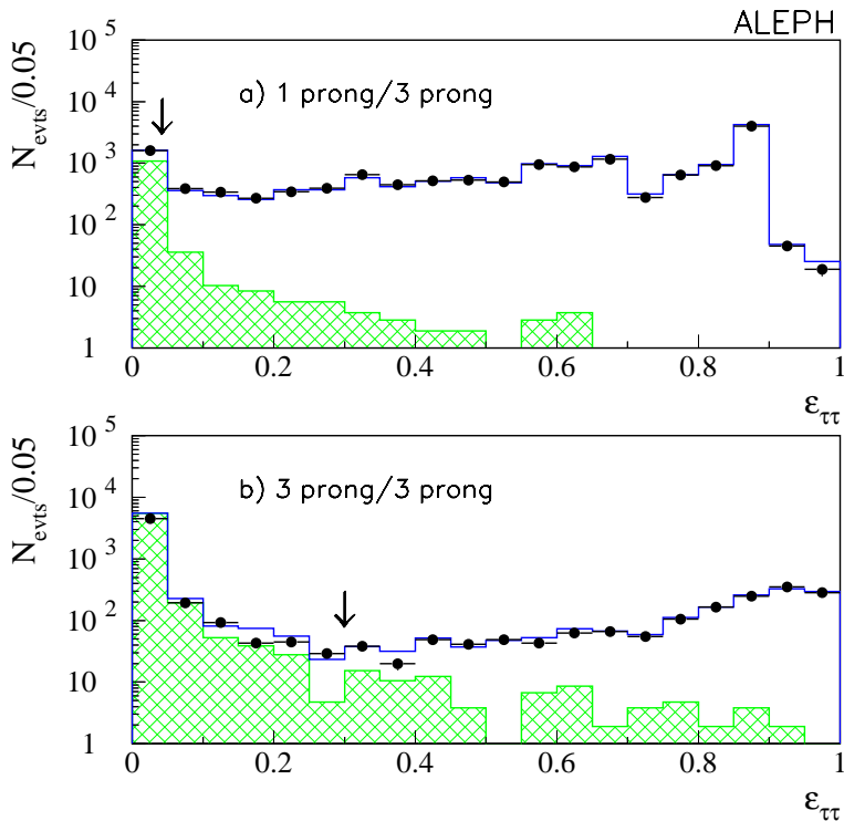
Fig. 14a,b. Global selection: distribution of the normalised estimator \mathcal{E}_{\tau+\tau^-} in a one-prong/three-prong events and b three-prong/three-prong events. The points represent the data, the open histogram the \tau^+\tau^- Monte Carlo and the hatched histogram the q\bar{q} Monte Carlo. The arrows indicate the position of the cuts
