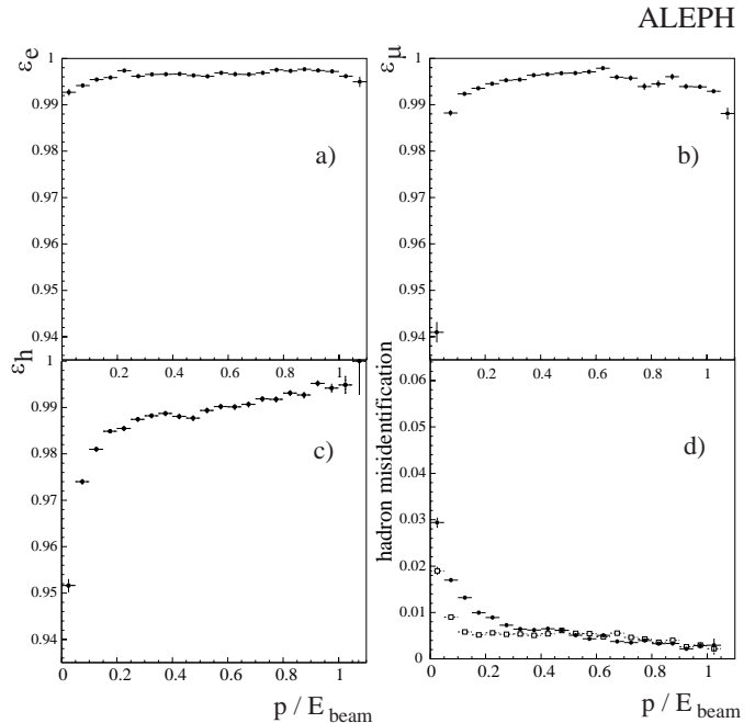
Fig. 1a–d. Identification efficiencies for electrons a , muons b and hadrons c as a function of the momentum to beam energy ratio. In d the probability for a hadron to be misidentified as an electron (squares) or a muon (circles) is shown. These distributions are obtained from a Monte Carlo simulation of electron, muon and tau dileptons and two-photon events
