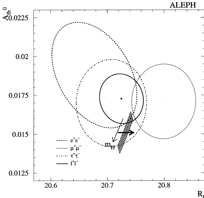
Fig. 23. The peak asymmetry vs the ratio of hadronic and lepton widths for all lepton species separately and assuming lepton universality. Shown are the one- \sigma contours (39.3% CL). The shaded area shows the Standard Model expectation for M_t = 174 \pm 5 \text{ GeV}/c^2 and 90 < M_H/\text{GeV}/c^2 < 1000 ; the horizontal arrow shows the change if the strong coupling constant is varied within \alpha_s(M_Z) = 0.119 \pm 0.002
