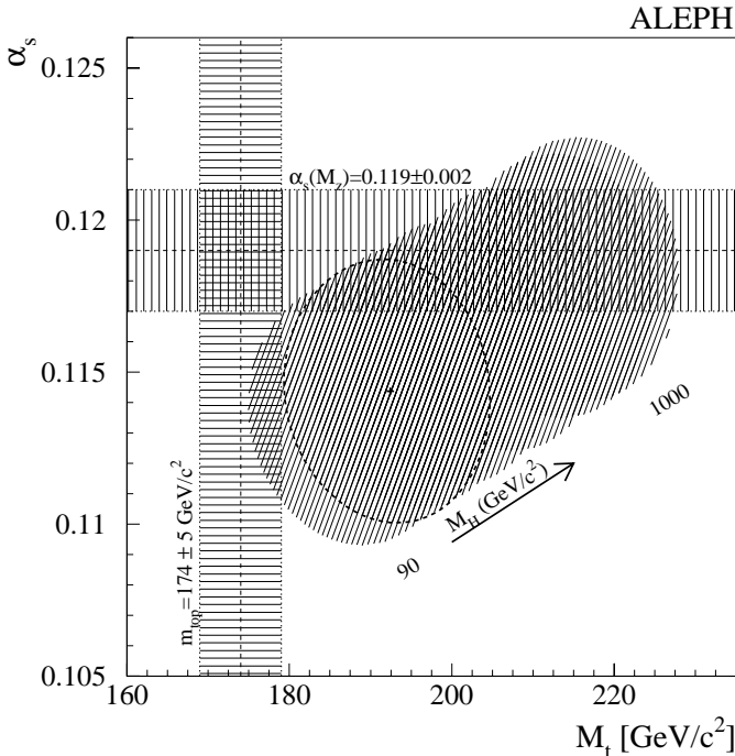
Fig. 25. One- \sigma contour lines in the plane of the top quark mass versus the strong coupling constant, for M_H = 150 \text{ GeV}/c^2 . The horizontal and vertical bands represent the world averages of other measurements. The shaded area indicates variations of the Higgs boson mass between 90 \text{ GeV}/c^2 and 1000 \text{ GeV}/c^2
