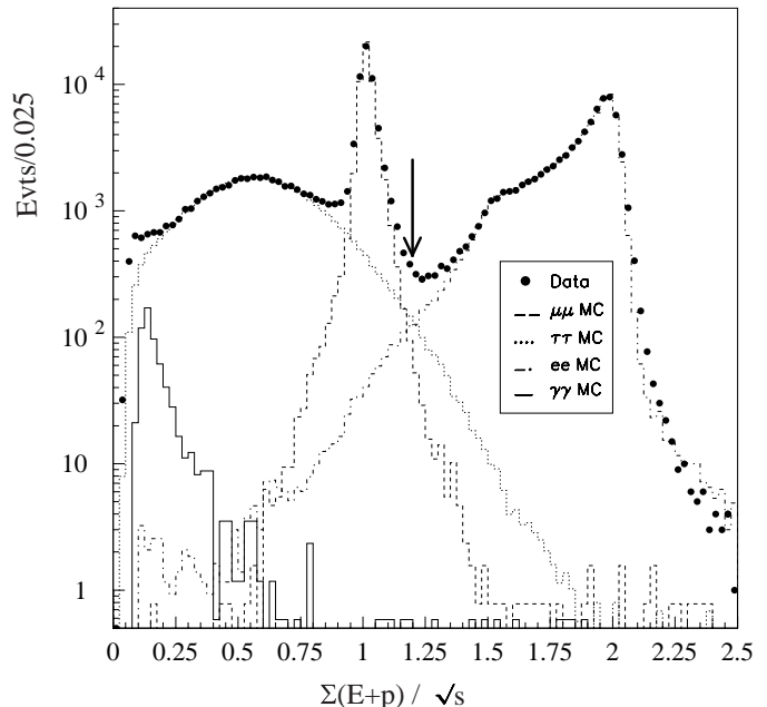
Fig. 11. Exclusive e^+e^- selection: distribution of the sum of energy and momentum of lepton pair events, normalised to the centre-of-mass energy, for data and Monte Carlo before muon identification cuts
