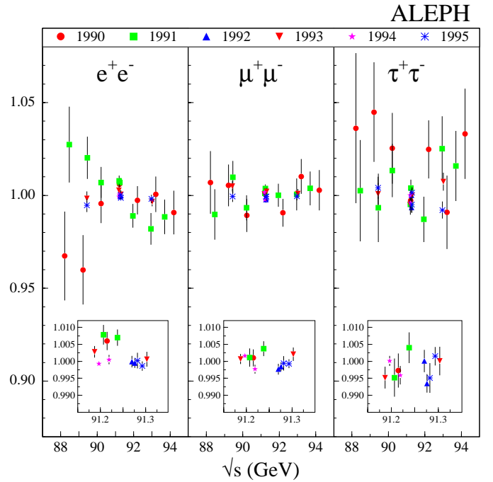
Fig. 18. Comparison of dilepton analyses: ratio of exclusive to global cross section for the three lepton species. Only errors from uncommon statistics are shown
