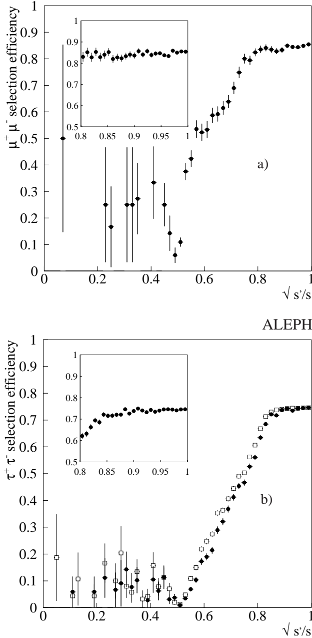
Fig. 19a,b. Overall efficiency as a function of \sqrt{s'}/s for the a muon and b tau selections. The white squares in b indicate the contribution of the acollinearity cut alone; to facilitate the comparison, this contribution has been normalised to have the same content in the last bin as the total efficiency. The inserts show an enlargement of the regions 0.8 < \sqrt{s'}/s < 1
