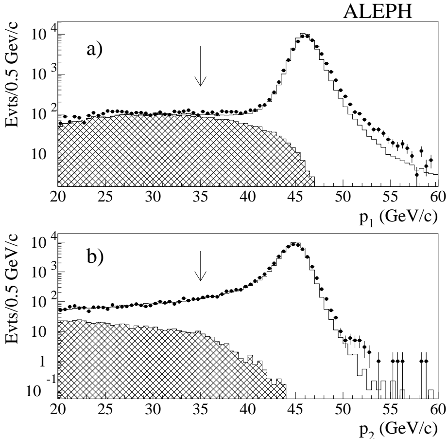
Fig. 9a,b. Exclusive \mu^+\mu^- selection: distribution of a the momentum p_1 of the leading track in events that fulfil the acceptance cuts and b the momentum p_2 of the second fastest track in events that fulfil the p_1 cut. Only events with at least one identified muon are plotted here. The arrows indicate the applied cuts. Dots are the data, the open histogram is the Monte Carlo for signal plus background and the hatched histogram is the \tau^+\tau^- Monte Carlo
