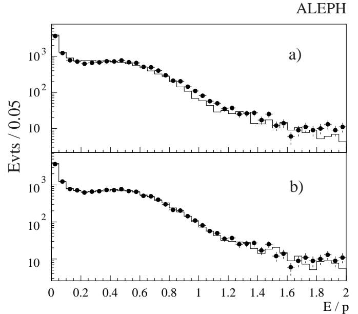
Fig. 12a,b. Exclusive e^+e^- selection: energy deposited by topologically selected pions in the ECAL divided by the hadron's momentum, a before energy correction and b after energy correction. Points represent the data, and the histogram is the Monte Carlo
